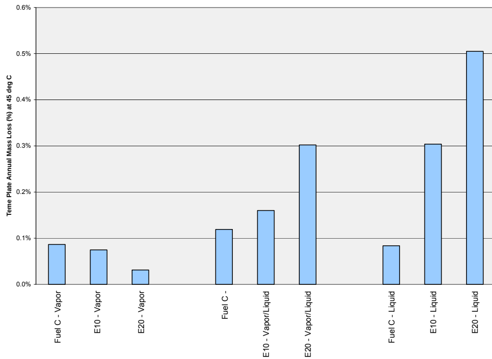
Figure 8.3.3: Terne Plate Mass Loss Rate
