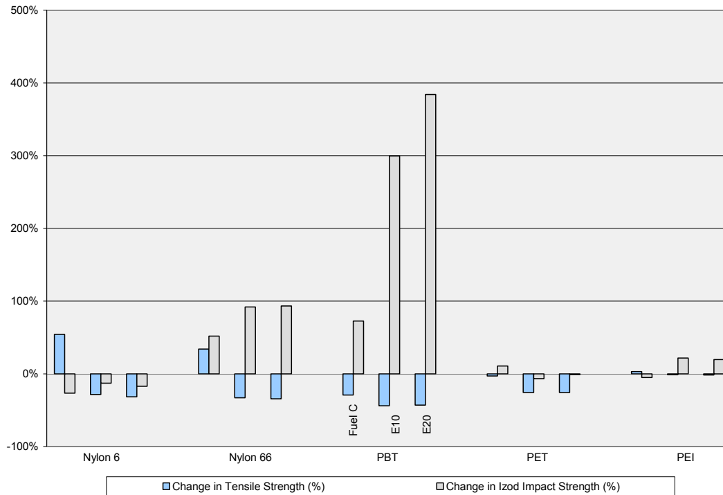
Figure 8.2.2: Plastic Tensile Strength and Izod Impact Strength
